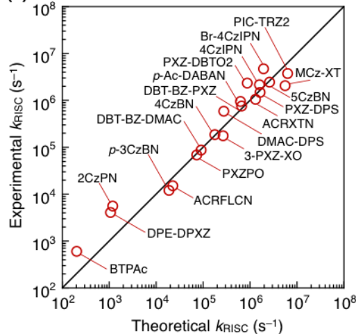
図 2. (a) Molecular structures of the examined thermally activated delayed fluorescence (TADF) materials categorized by their rate constants of reverse intersystem crossing ( k_{\text{RISC}} ). (b) Comparison of the experimental and theoretical k_{\text{RISC}} .
