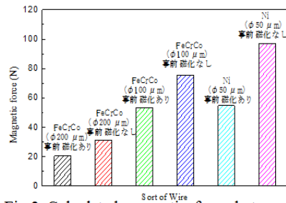
Fig.2 Calculated magnetic force between magnetic wire and permanent magnet in
