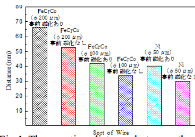
Fig.1 The reaction distance between the magnetic wire and permanent magnet.
